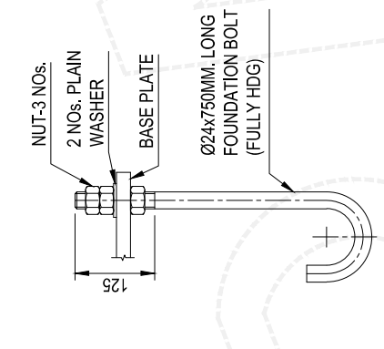
FOUNDATION BOLT DETAIL
