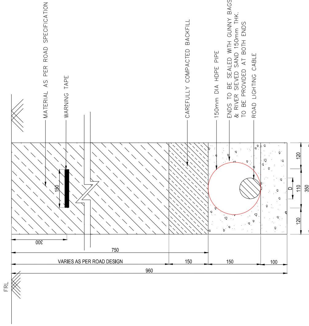
TYPICAL ROAD LIGHTING CABLES LAYING ARRANGEMENT FOR ROAD CROSSING
