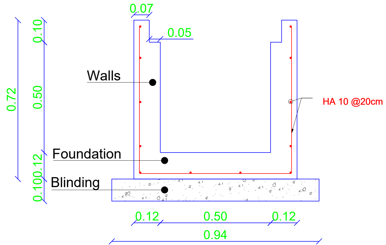
TYPICAL DRAIN SECTION FOR (50x50cm)
