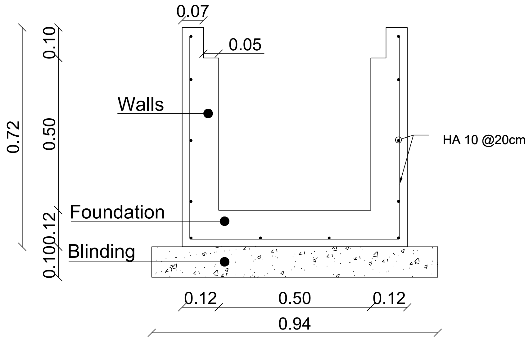
TYPICAL DRAIN SECTION FOR (50x50cm)
